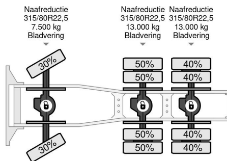
MAN 33.463 DFS 6x6 FULL SPRING SUSPENSION TRACT...
