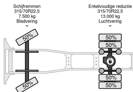
DAF XF 105.460 SPACECAB (ZF16 MANUAL GEARB... 4x2
