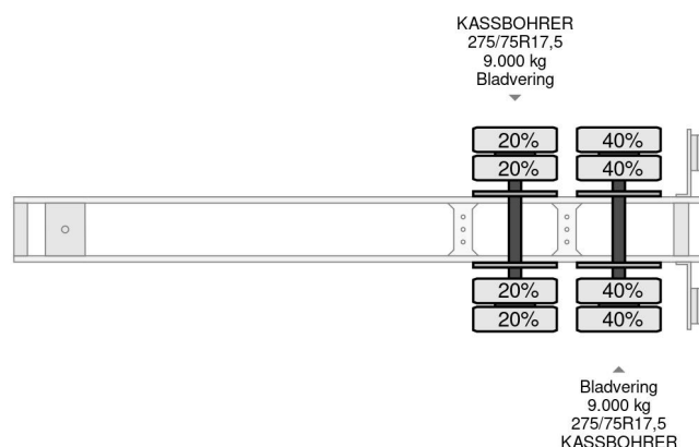
GT Trailers ETC 0027-01 2-AXLE STEEL SUSPENSION MA...
