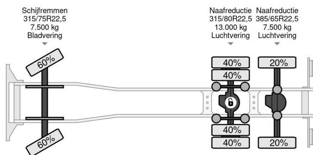
MAN 26.414 FNL-T (6-CILINDERHEADS) 6x4 CHASSIS (EU...
