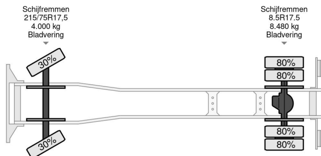
Renault Midlum 180 4x2 FULL STEEL SUSPENSION CHASSIS...
