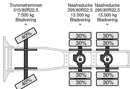
Renault R385 Major 6x4 SPRING SUSPENSION/LAMME (ZF... Referentienummer: SN 59970039 Z
