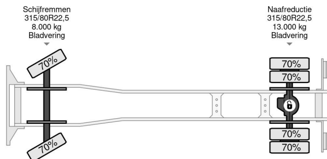
Mercedes-Benz Actros 2031 K WITH PALFINGER PK11... 4x2
