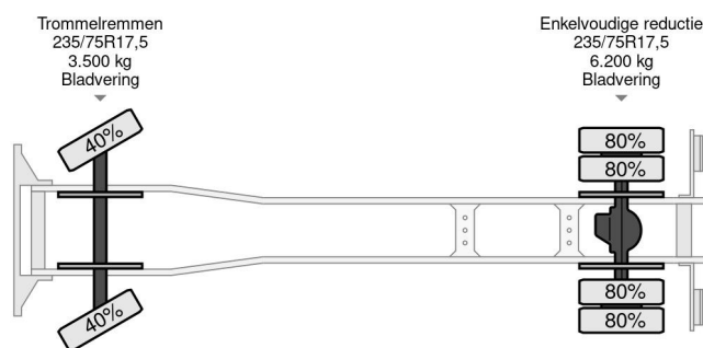
Mercedes-Benz LK 914K (6-CILINDER) FULL STEEL C... 4x2
